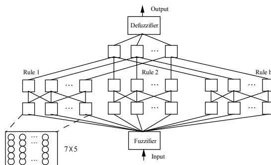
Fig. 9. Network architecture for module development.
