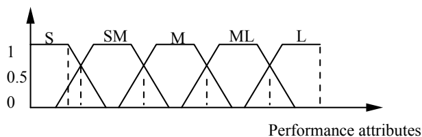
Fig. 10. Membership function of a fuzzy set \{S, SM, M, ML, L\} .
