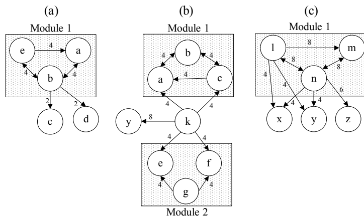
Fig. 6. Modularity represented by graphs: (a) function-swapping modularity, (b) function-sharing modularity, and (c) bus modularity.
